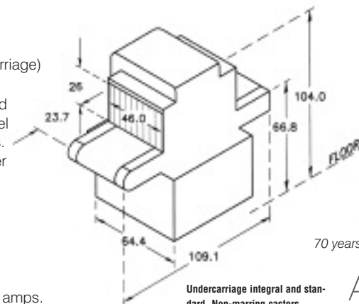
Dimensions are in centimeters Note: Non-marring casters
